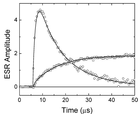
Figure 1. Kinetic traces of the central lines of the precursor and successor radicals. A N 2 -saturated aqueous solution of 0.1 M 2-propanol, 0.4 M acetone, and 25 mM sodium nitrite with 1 mM phosphate buffer (pH 7) was used. The open circles show the kinetic trace of the (CH 3 ) 2 C • -OH radical at \Delta B_0 = -4.77 G, and the square points show the kinetic trace of the [HO-C(CH 3 ) 2 NO 2 ] •- radical at \Delta B_0 = -8.10 G. Solid lines represent simulations as described later in this work. The vertical scale is given in arbitrary units, but the relative amplitudes of the two curves are as observed.
